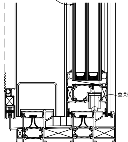
1 VERTICAL SECTION DETAIL A-A'
