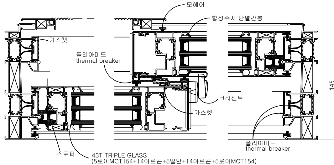
2 HORIZONTAL SECTION DETAIL B-B'
