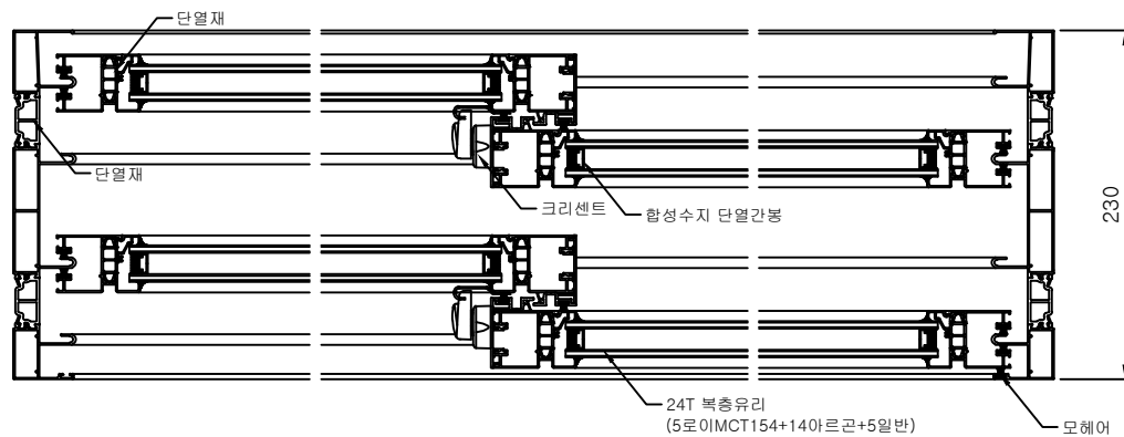
2 HORIZONTAL SECTION DETAIL
