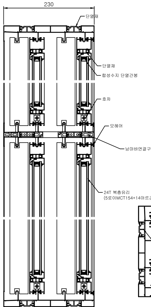
1 VERTICAL SECTION DETAIL
