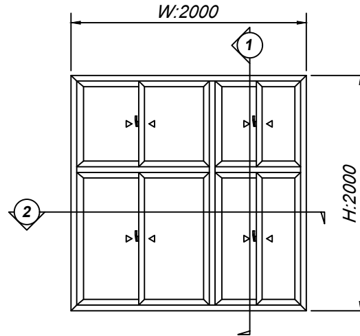
INSIDE ELEVATION
