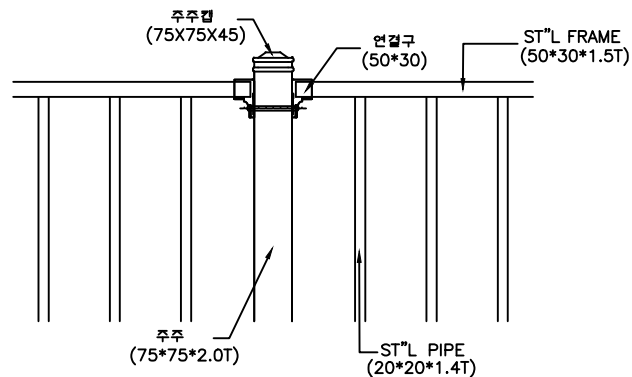
ASSEMBLY "DETAIL" SCALE:NONE
