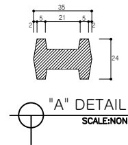
Base Plate Detail SCALE: NONE
