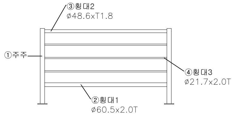
Fence DETAIL SCALE:NONE
