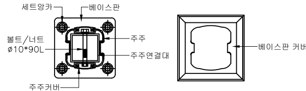
Base Plate Detail SCALE: NONE
