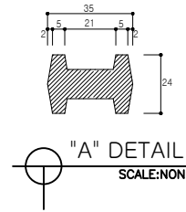
Base Plate Detail SCALE:NONE
