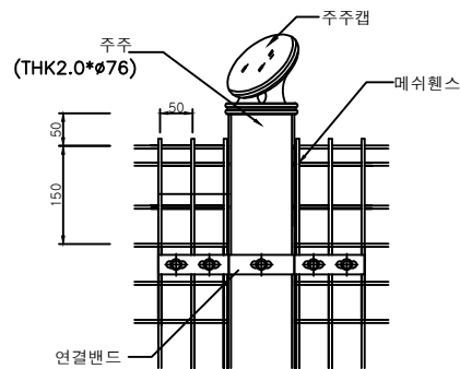
"A" DETAIL
