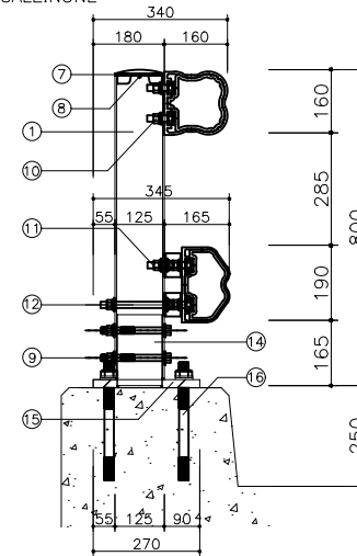
SECT DETAIL "A"
